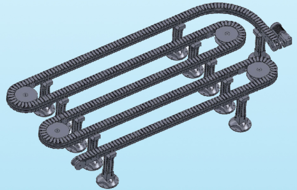
Double Rail
