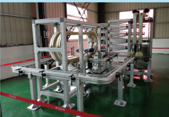
Flexible Chain System
